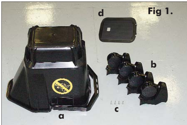
Fig 1. COMPONENTS CHECK.
